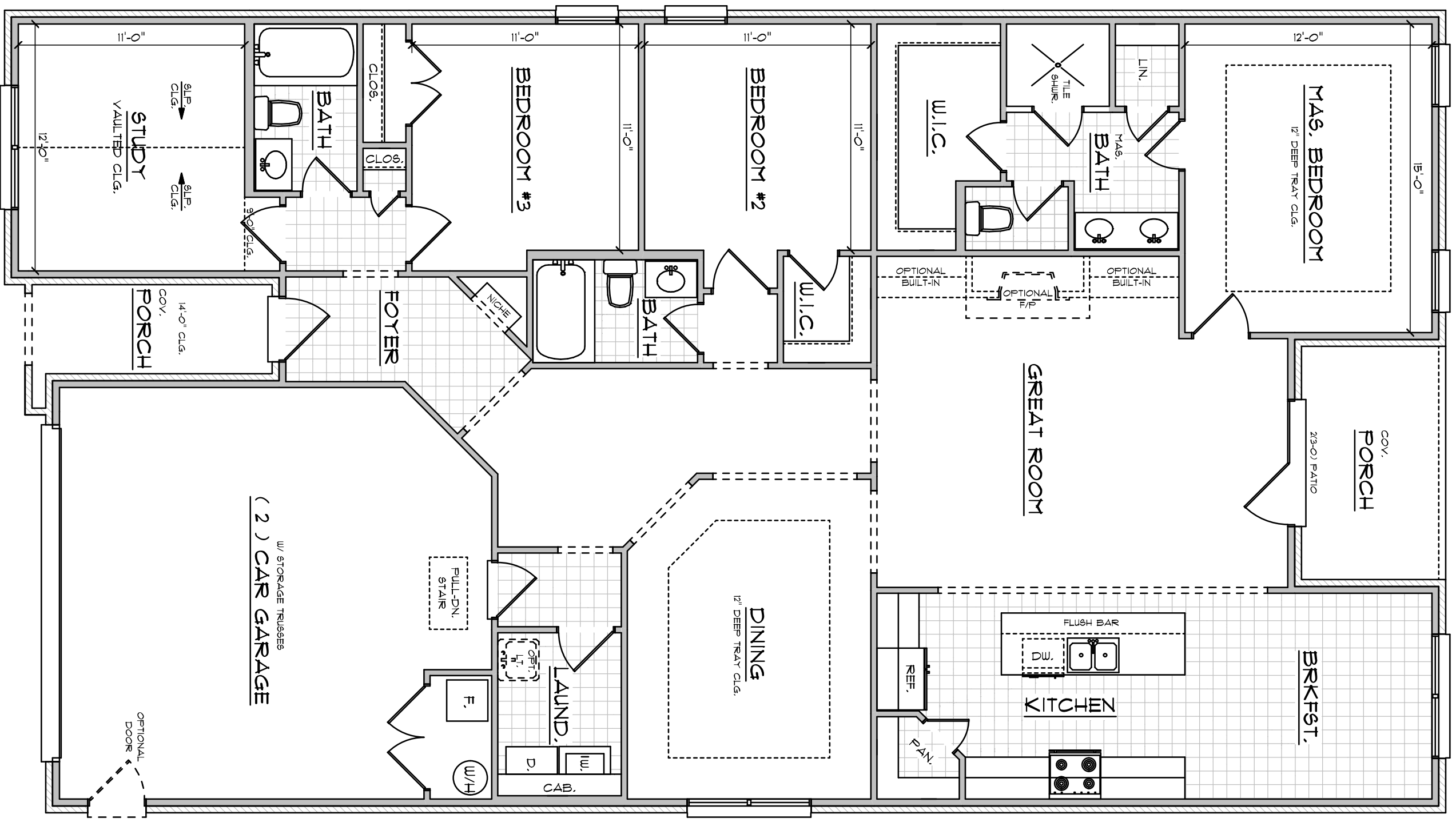
FLOOR PLAN "B"
