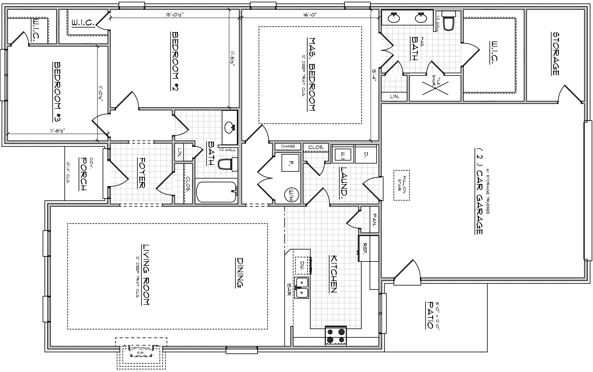
FLOOR PLAN
